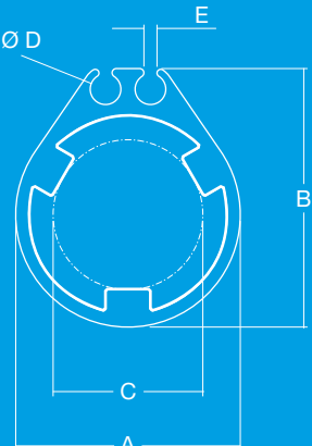
FOIL WITH EXPANDING OPENABLE CONNECTOR
